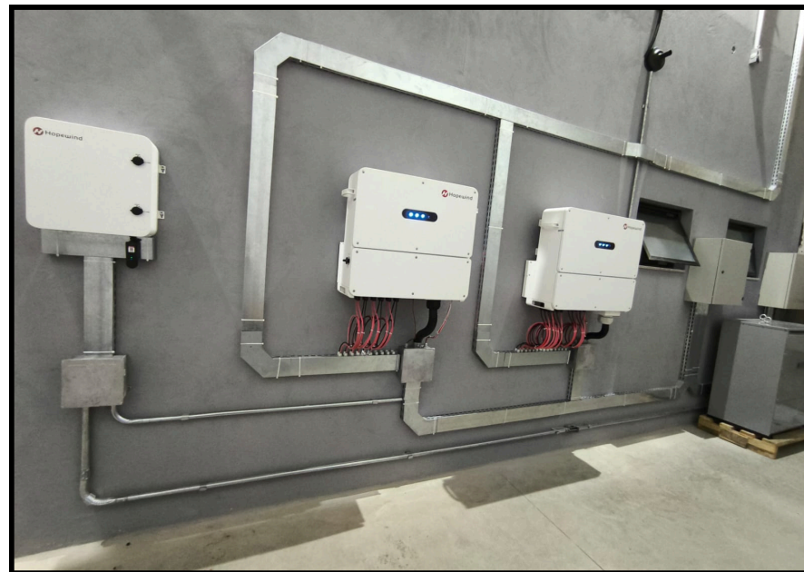
Projeto Grid 0 industrial 165kwp
